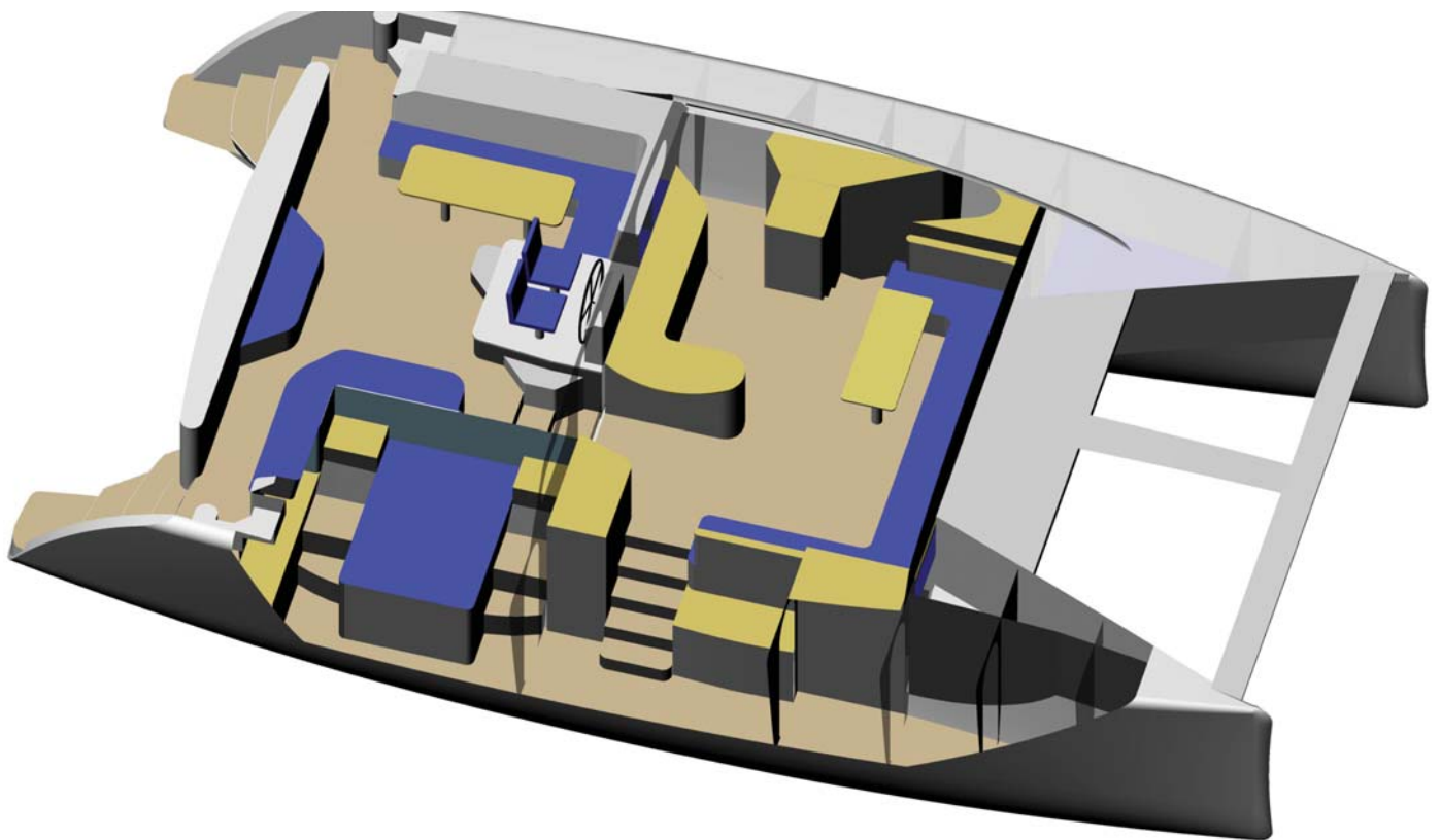
FreeFlow 46 Interior layout showing owners starboard hull island queen size berth aft, bathroom forward – port side queen size berth aft, central bathroom and shower area with another queen size berth or two singles forward.
